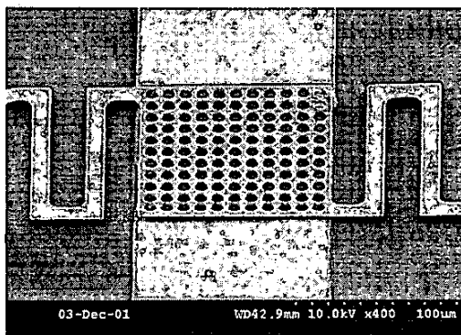
Fig. 4: SEM of a low actuation voltage meander-shaped support switch. The air-gap is 2μm.
