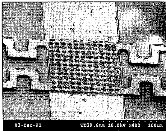
Fig. 3: SEM of a fabricated bridge-type CPW switch with 1μm thick Cu membrane and 4 meander-shaped supports. The size of the membrane is 120μm×120μm.
