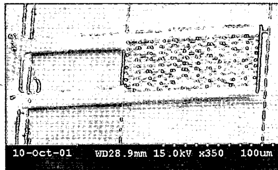
Fig. 6: SEM view of a switch with 1μm thick membrane fabricated after the ground posts were electroplated.
