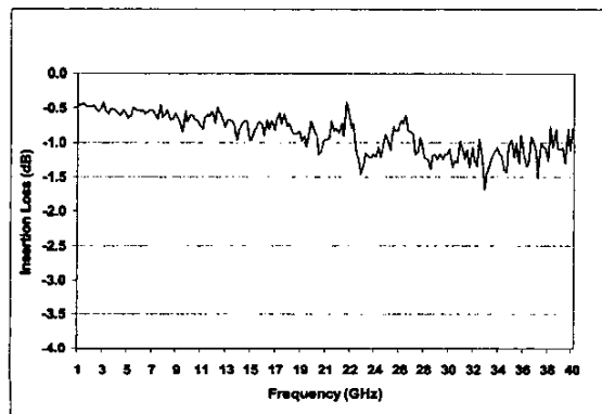
Fig. 8: Measured insertion loss of the thru line only.
